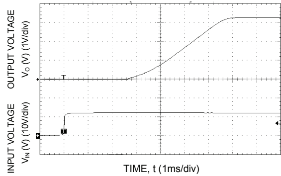
Figure 16. Typical Start-Up with application of V_{in} ( V_{in} = 12.0Vdc , V_o = 3.3Vdc , I_o = 3A ).
