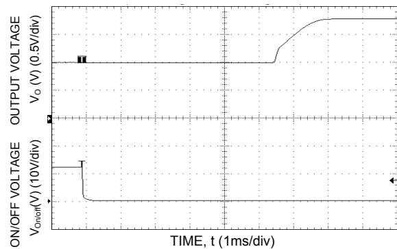
Figure 17 Typical Start-Up Using Remote On/Off with Prebias ( V_{in} = 12.0Vdc , V_o = 1.8Vdc , I_o = 1.0A , V_{bias} = 1.0Vdc ).
